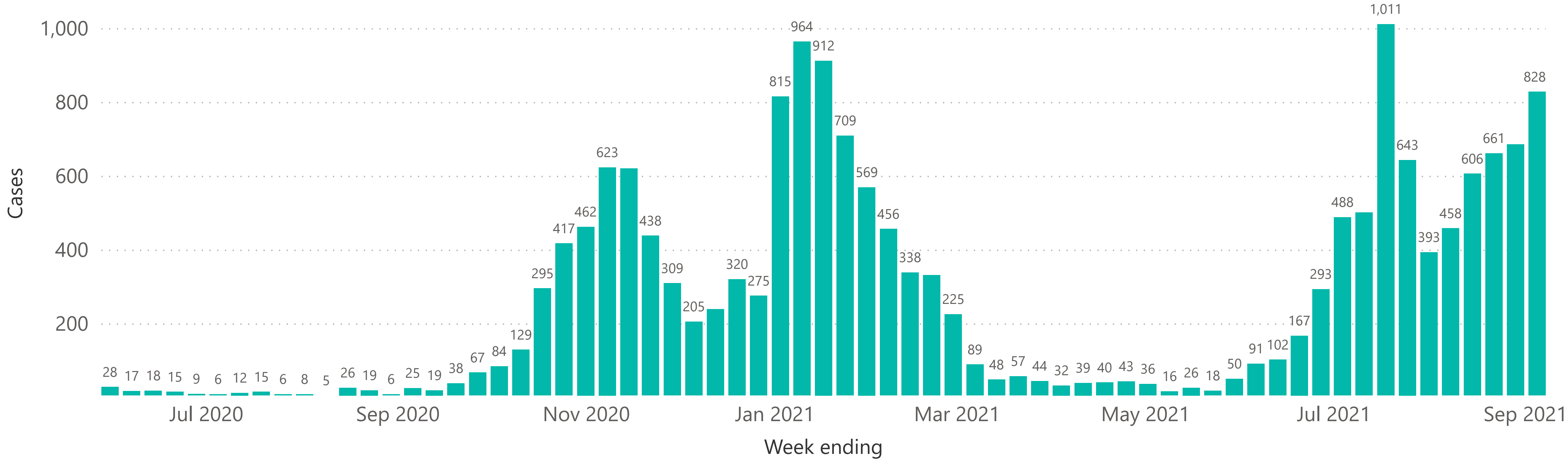
Telford and Wrekin total weekly COVID-19 cases
