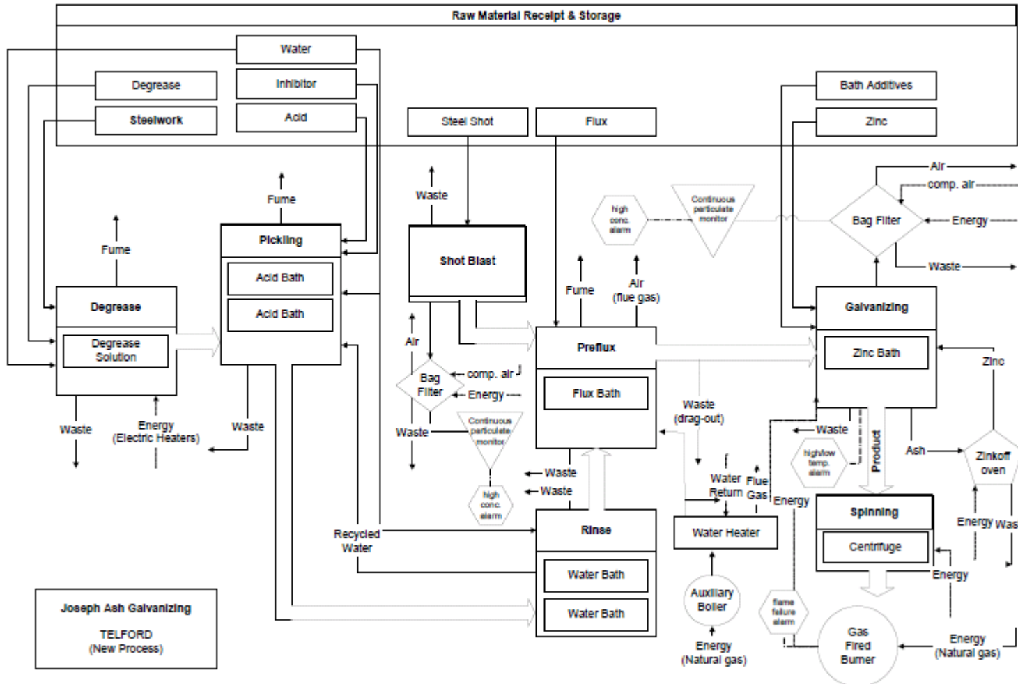
Joseph Ash Galvanizing Telford (New Process)– Process Flow Diagram
