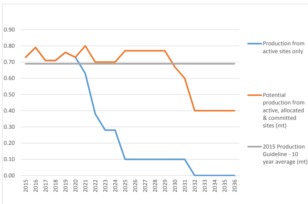
Figure 14: Assessment of Future Sand & Gravel Productive Capacity in Shropshire 2016 - 2036
