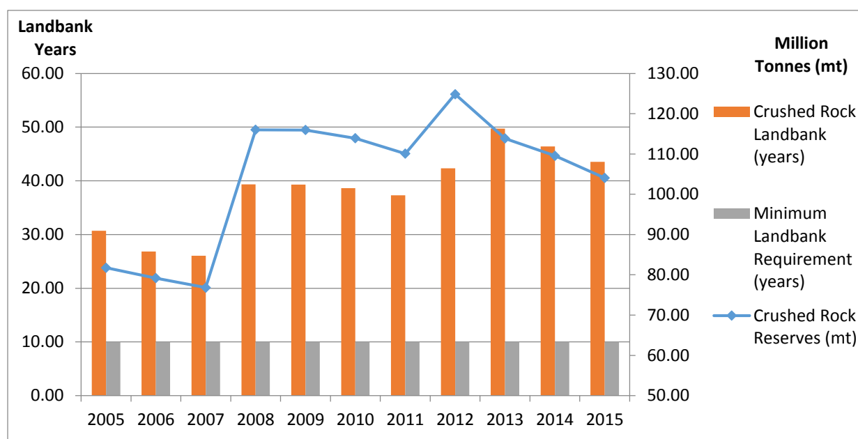
Figure 13: Shropshire Crushed Rock Reserves and Landbank 2005-2015
